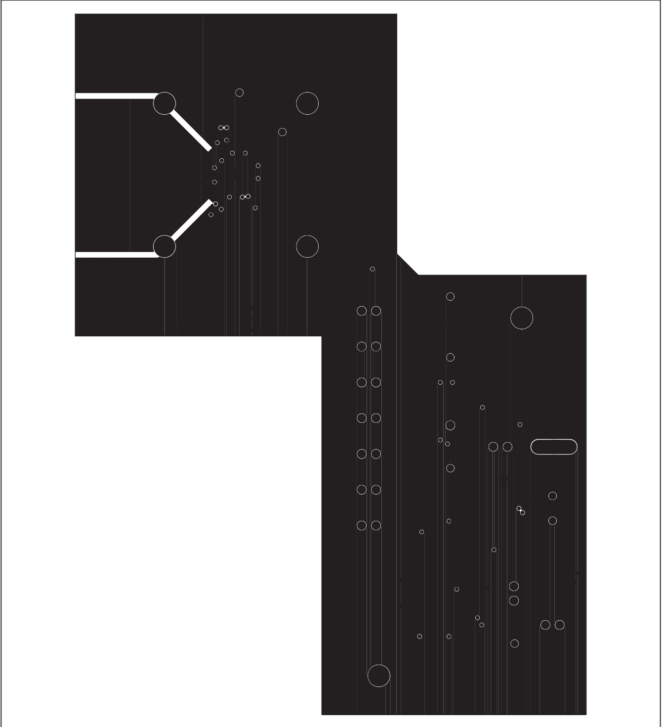
Figure 6. MAX3799 EV Kit PCB Layout—Ground Plane
