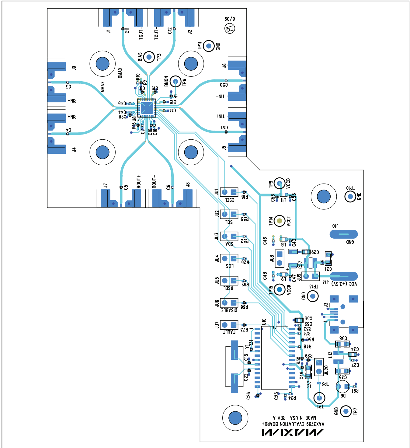
Figure 4. MAX3799 EV Kit Component Placement Guide—Component Side
