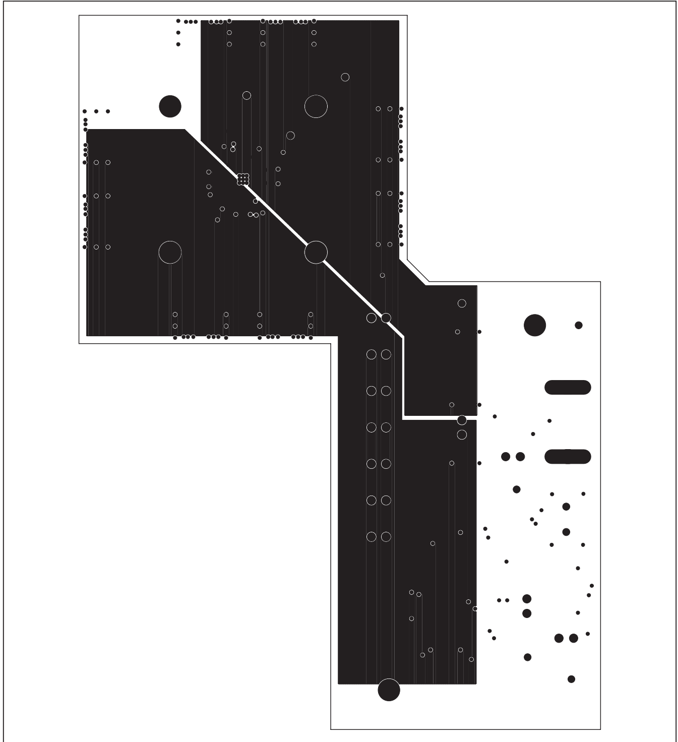
Figure 7. MAX3799 EV Kit PCB Layout—Power Plane
