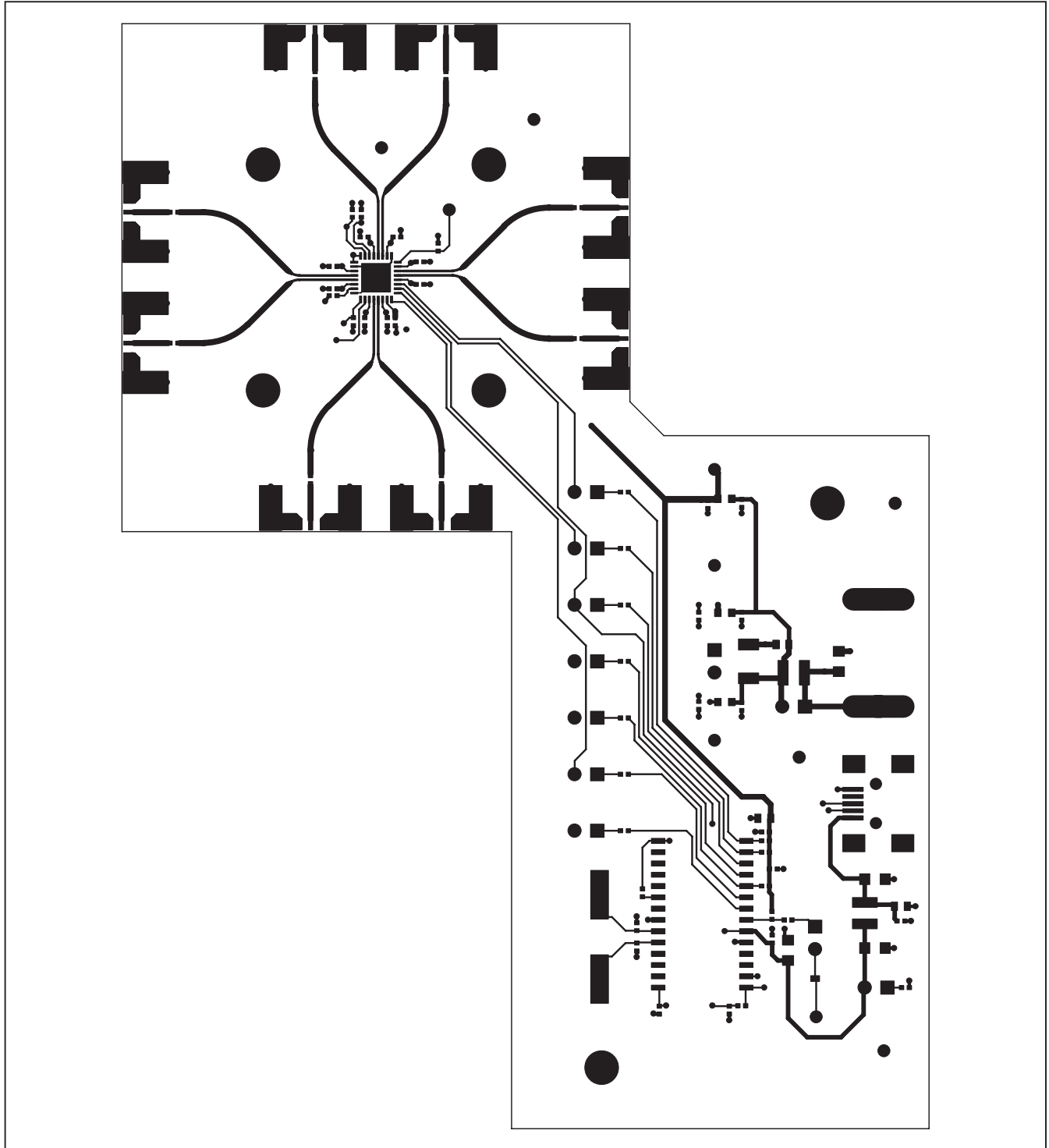
Figure 5. MAX3799 EV Kit PCB Layout—Component Side
